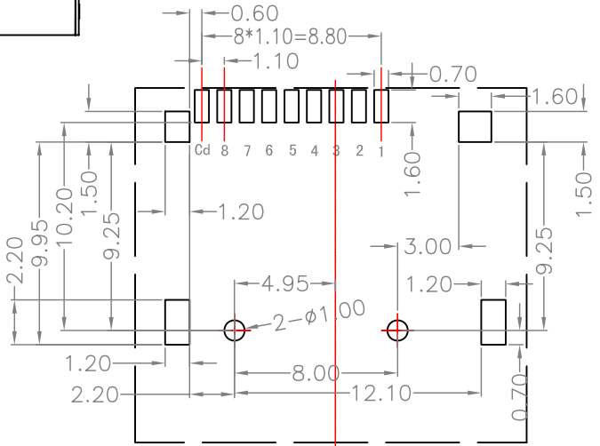
RECOMMENDED P. C. B HOLE LAYOUT COMPONENT SIDE VIEW (TOLERANCE: +/-0.05)
