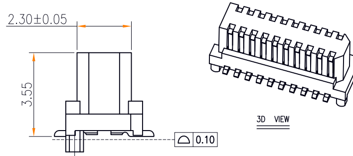
MATING HEIGHT SCALE: 1.25:1
